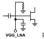
Figure 9. VGG_LNA Interface Schematic
