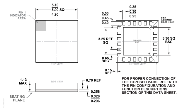
Figure 92. 24-Terminal Land Grid Array [LGA] (CC-24-8)
